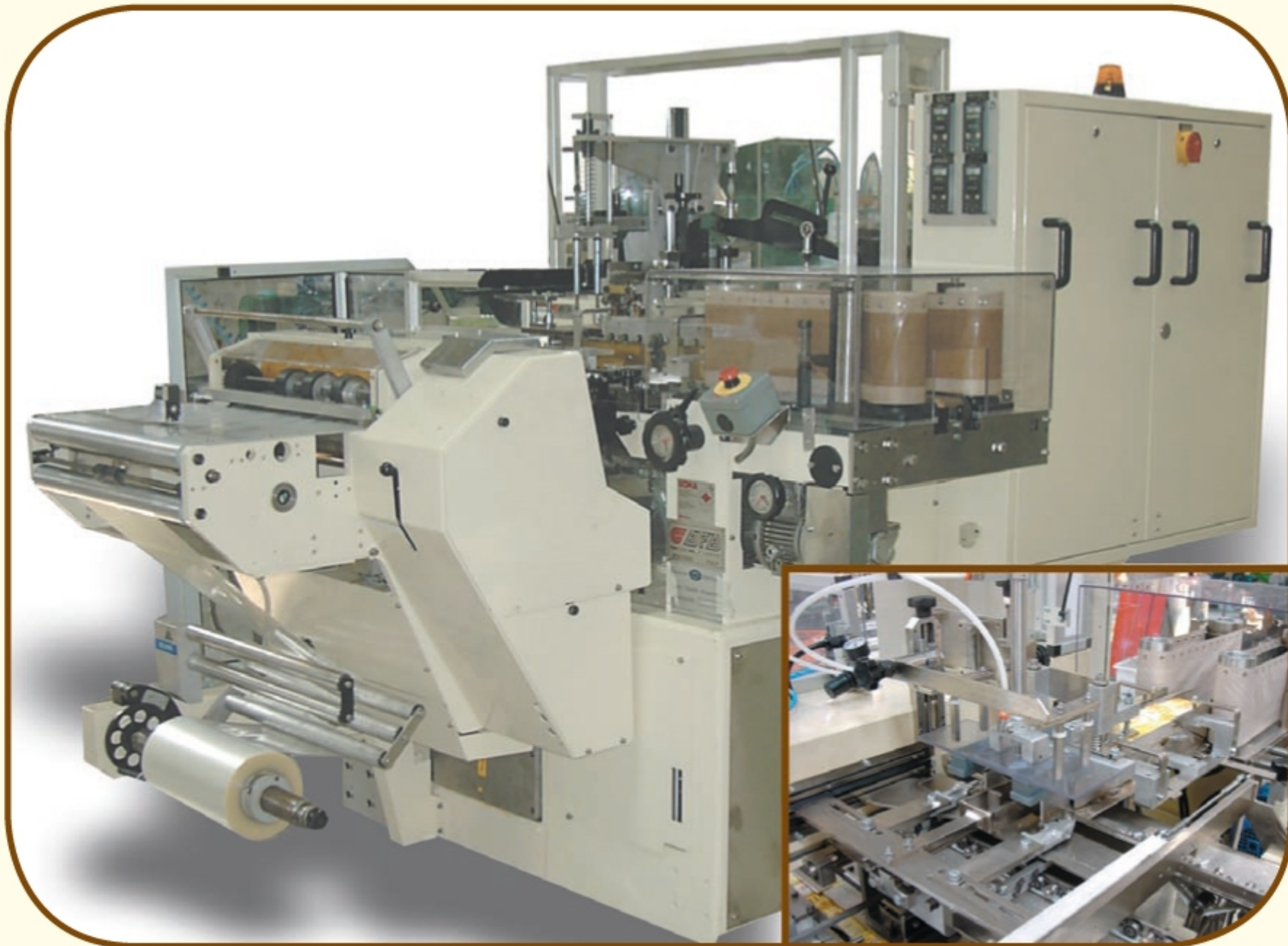
Rebuilt BFB 3711 Bundler
