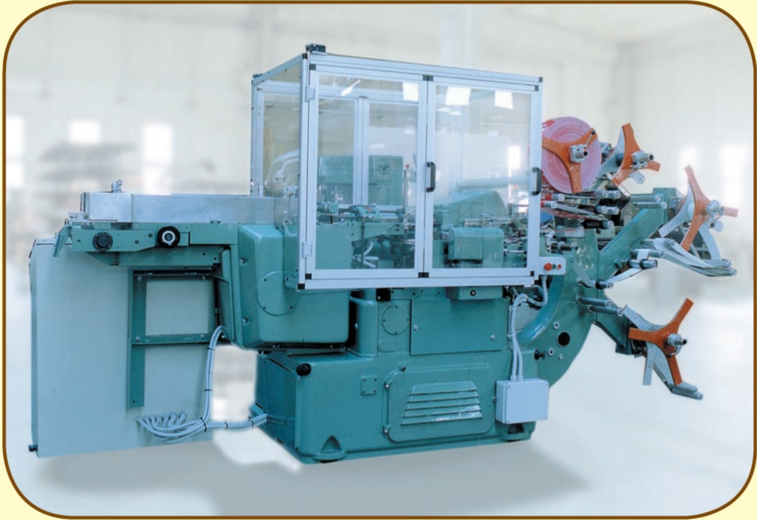
Rebuilt ACMA 711 Wrapper
